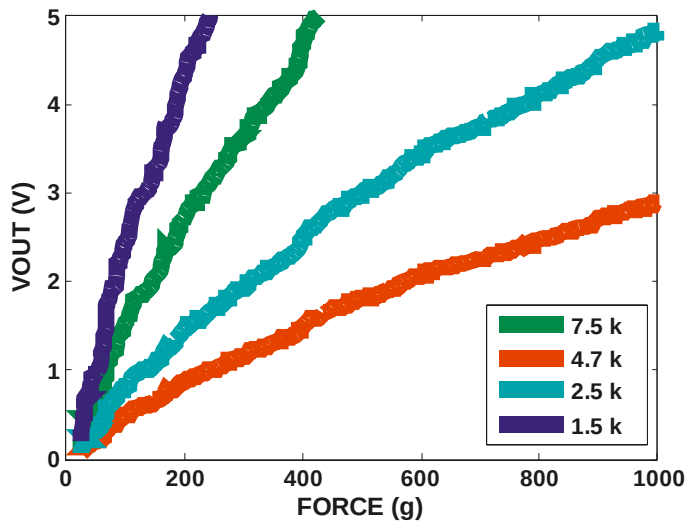
Figure 14: FSR Current-to-Voltage
