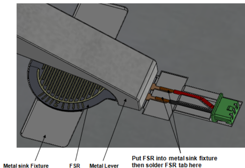
FSR Soldering Fixture
